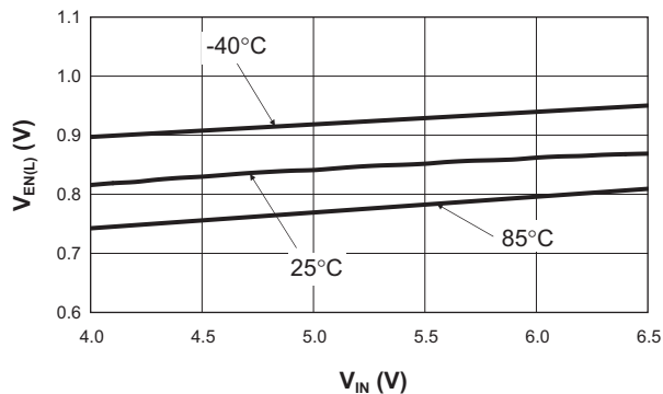
Enable Threshold Low vs. Input Voltage ( R_{SET} = 8.06k\Omega )
