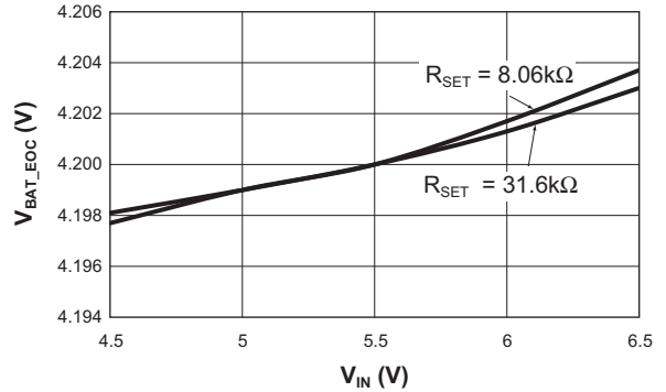
End of Charge Battery Voltage vs. Input Voltage vs. Input Voltage
